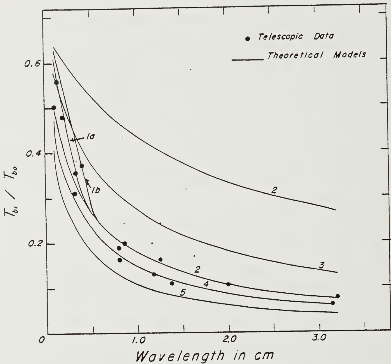
Ratio of the amplitude of variation to the mean brightness temperature over a lunation vs wavelength. The curves 1-7 are results of theoretical calculations based on Apollo 15 thermal properties and 7 different dielectric property profiles. 1) data of Bassett and Shackelford (1972). 2) \ell_\lambda = \lambda , 3) \ell_\lambda = 3\lambda , 4) \ell_\lambda = 8\lambda . 5) \ell_\lambda = 12\lambda . Curves 1a used the results of Ade et al., 1971 and 1b the results of Clegg et al. (1972) for \lambda = 0.1 - 0.2 .
